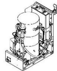
DR4180 WATER HEATER UP-RIGHT WITH COVER REMOVED
