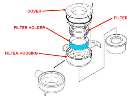
Water Separator Assembly
