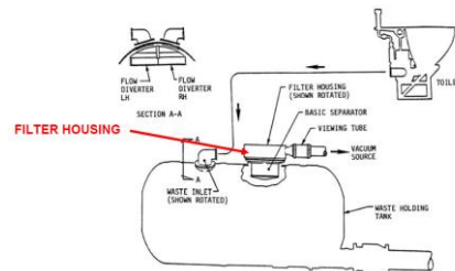
Waste Holding Tank System
